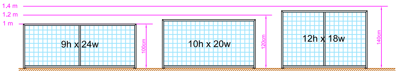
Large "Landscape" Racks
