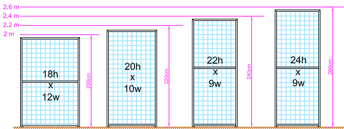
Large "Portrait" Racks
